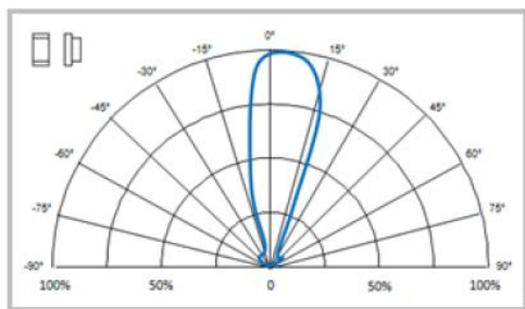
Relative Radiant Intensity vs Angular Displacement
