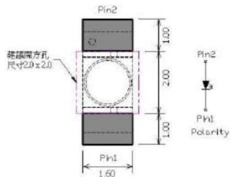
Figure 1. IN-S126ETIR Solder Pattern
