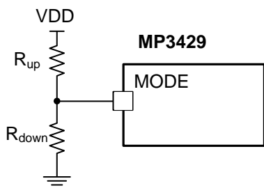
Figure 3: MODE Setting
