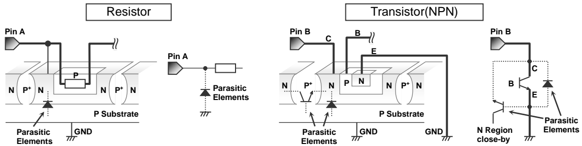
Figure 42. Example of IC structure
