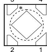
RP122K (DFN (PLP) 1010-4) Pin Configuration
