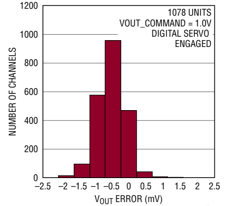
Typical LTC7883 Output Voltage Distribution at 105°C
