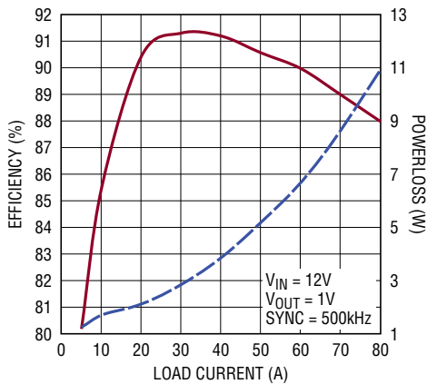
Efficiency and Loss vs Load (2-Phase Using FDMF5820DC DrMOS)
