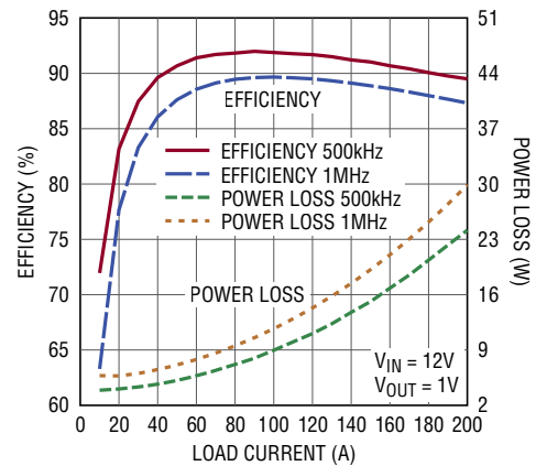
Efficiency and Loss vs Load (4-Phase Using LTC7051)
