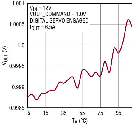
LTC7883 1.0V Regulated Output vs Temperature
