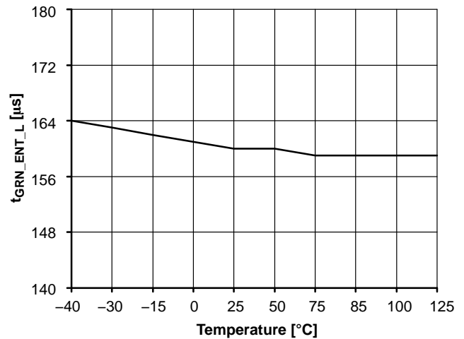
Figure 14. t_{GRN\_ENT\_L}
