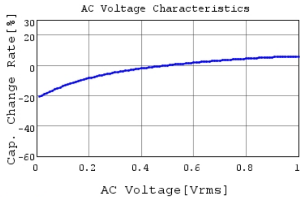
GRM31CD80J107MEA8 C-AC Voltage capchange, Dc
