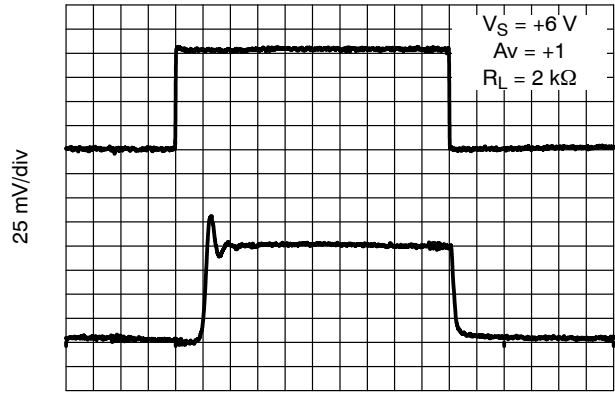
500 ns/div Figure 31. 6 V Non-Inverting Small Signal Pulse Response
