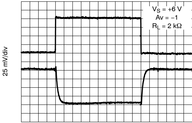
500 ns/div Figure 30. 6 V Inverting Small Signal Pulse Response
