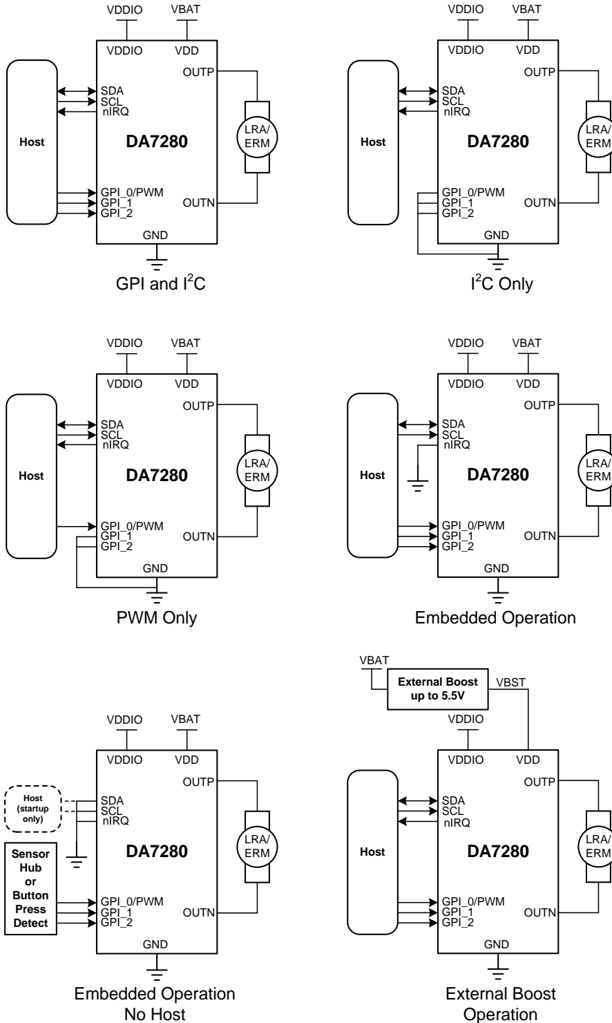
Figure 1: System Diagrams
