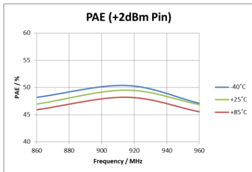
Figure 6: PAE (+2 dBm Pin)
