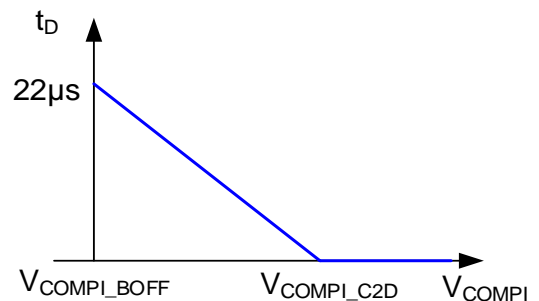
Figure 6: Dead Time Extension
