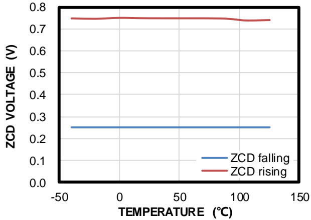
Zero-Current Detection Threshold vs. T_J
