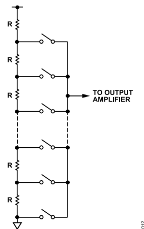
Figure 32. Resistor String
