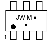
SC-74 CASE 318F STYLE 8
