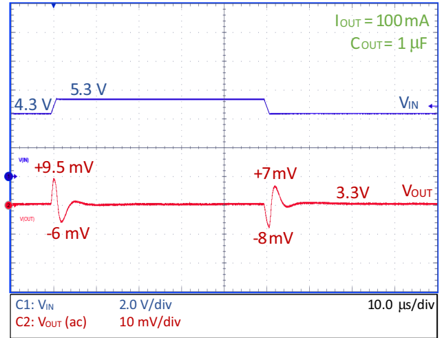
Figure 33. Line Transient – NCP730–3.3 V
