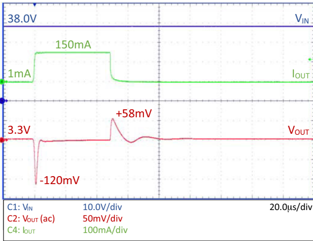
Figure 20. Load Transient – NCV8730–3.3 V, C_{OUT} = 1\text{ }\mu\text{F}
