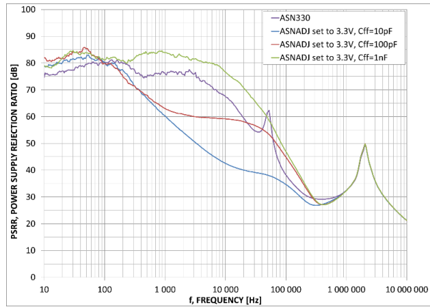
Figure 59. PSRR – Different C_{FF}
