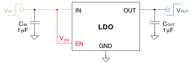
Figure 64. Circuit – EN Pin Connected to IN Pin
