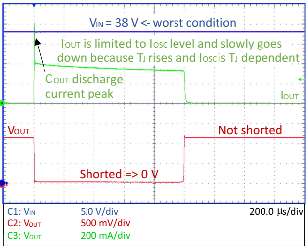
Figure 40. Output Short (1 ms) – NCP730–ADJ–1.2 V
