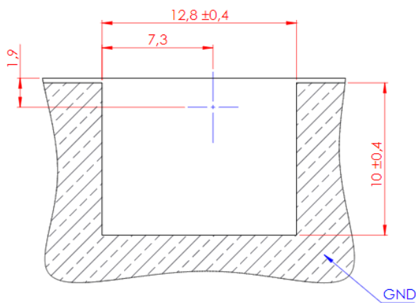
GROUND CLEARANCE BOTTOM VIEW (SILKSCREEN NOT SHOWN) SCALE 5:1
