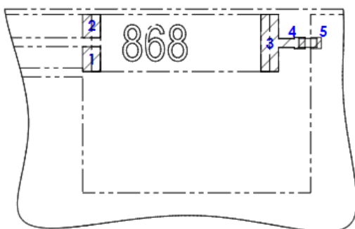
FOOTPRINT SOLDER PADS WITH PCB OUTLINE SCALE 5:1
