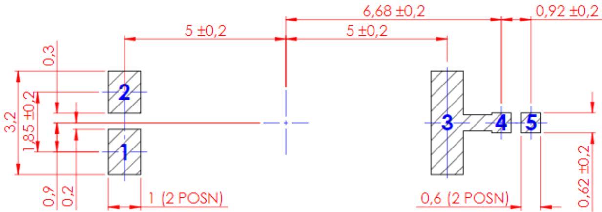
FOOTPRINT PCB
