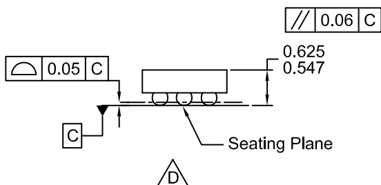
SIDE VIEWS
