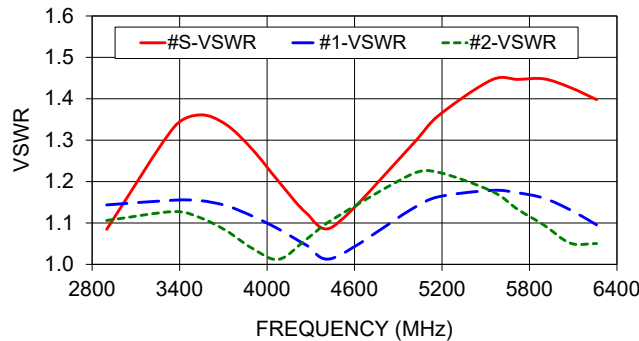
GP2X+ VSWR
