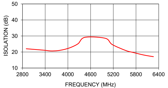
GP2X+ ISOLATION
