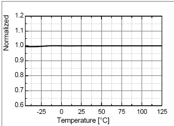
Figure 13. Zero Duty Cycle Output Voltage ( V_{E\Delta Z} ) vs. T_A
