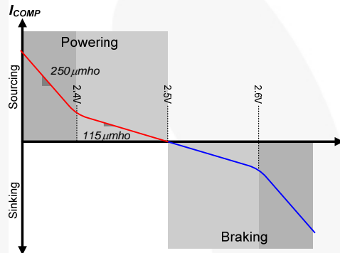
Figure 39. Gain Characteristic
