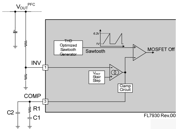
Figure 36. Control Circuit
