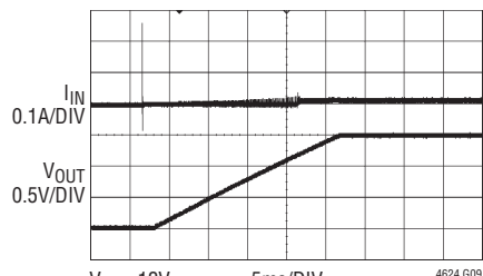
Start-Up with No Load
