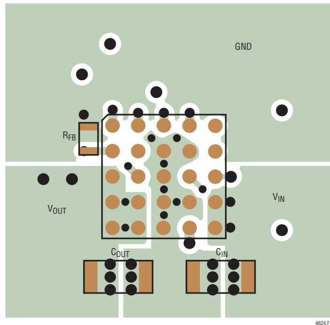
Figure 17. Recommended PCB Layout
