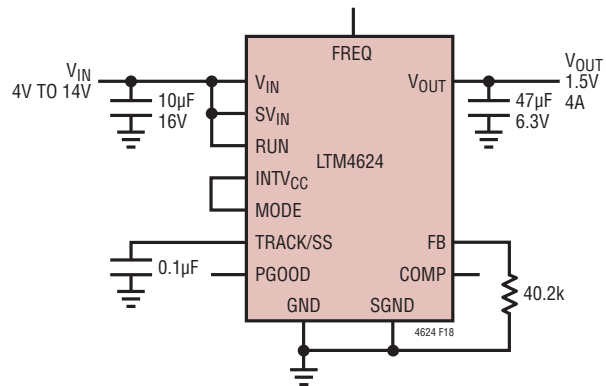
Figure 18. 4V_{IN} to 14V_{IN} , 1.5V Output at 4A Design
