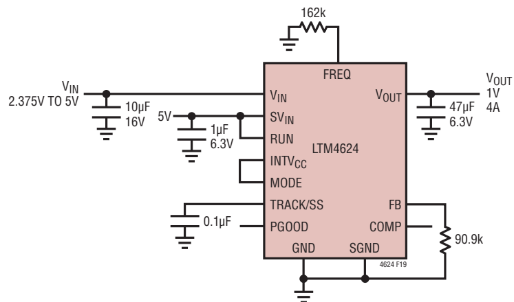
Figure 19. 2.375V_{IN} to 5V_{IN} , 1V Output with 2MHz Operating Frequency
