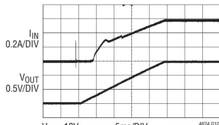
Start-Up with 4A Load
