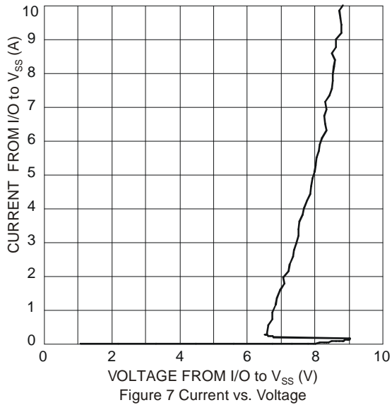
Figure 7 Current vs. Voltage
