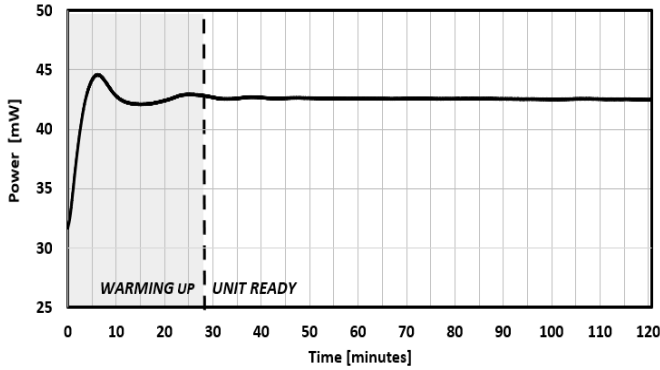
FIG. 15: WARM-UP TIME
