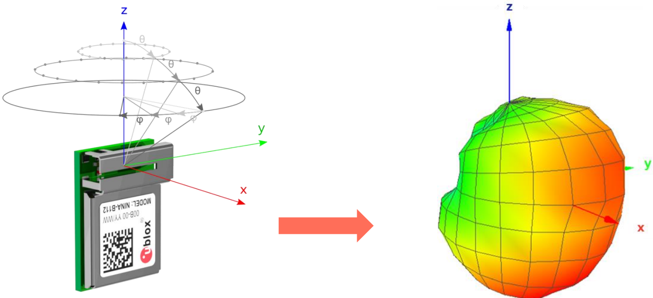
Figure 5: Measurement procedure for determining radiation patterns
