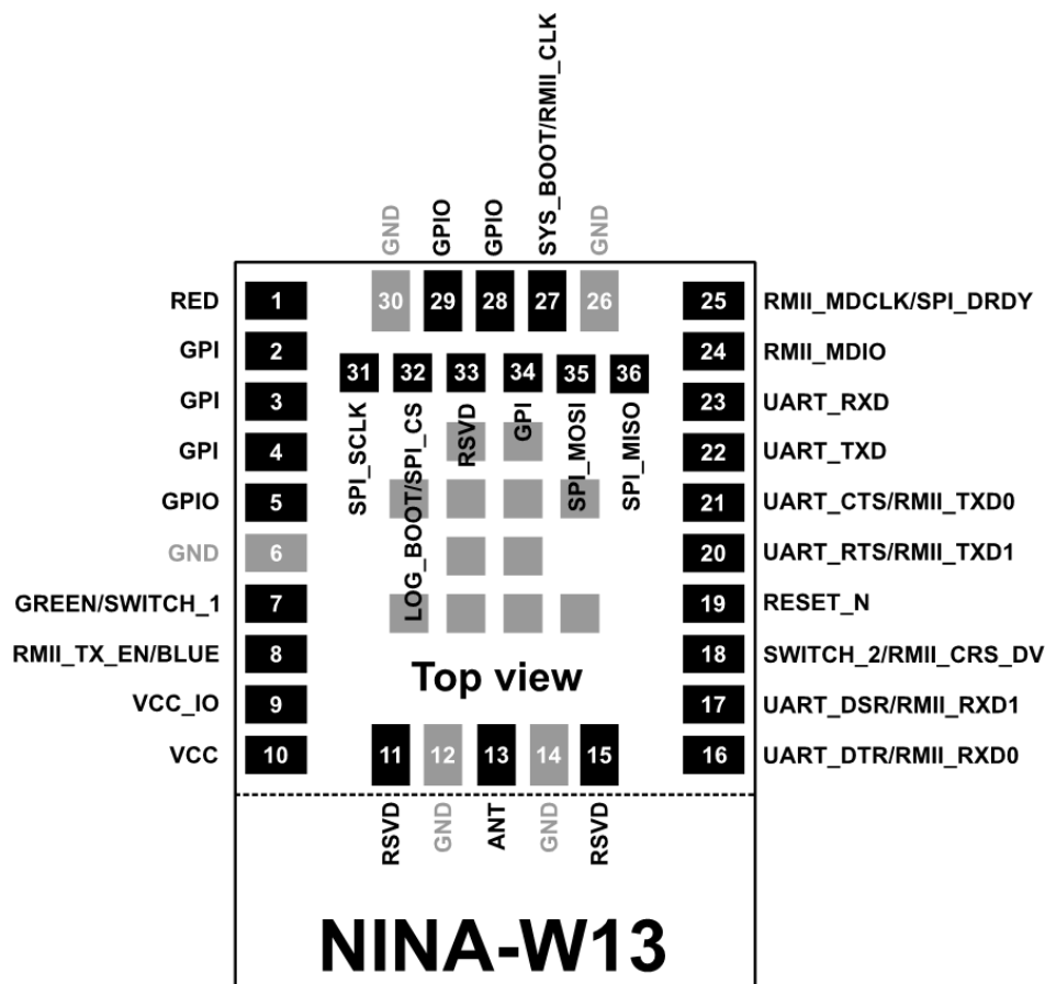
Figure 4: NINA-W13x pin assignment (top view)
