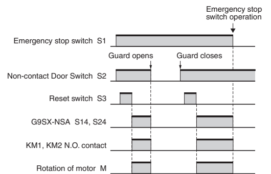
Timing chart
