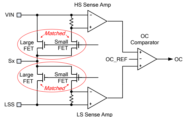
Figure 3: OCP Circuit
