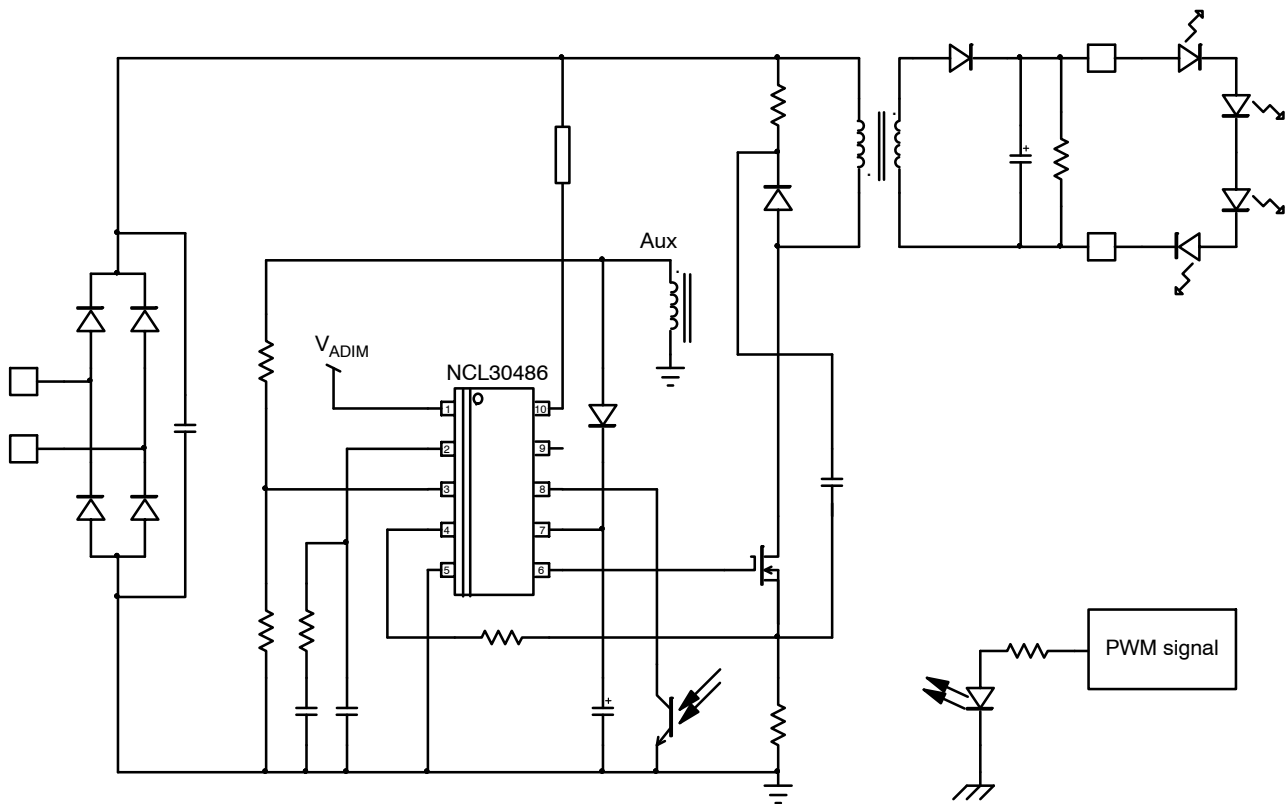
Figure 1. Typical Application Schematic for NCL30486B
