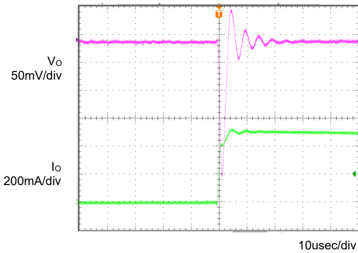
Fig.5 Transient Response (0→0.5A) Co=1µF, Ta=105°C
