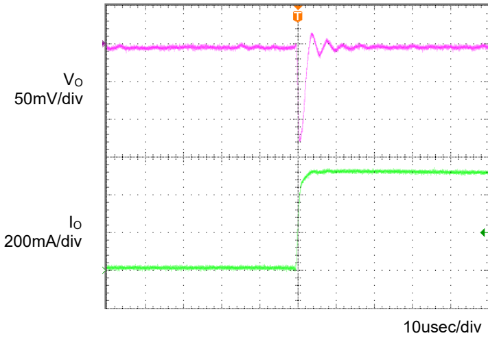
Fig.3 Transient Response (0→0.5A) Co=1µF, Ta=-40°C
