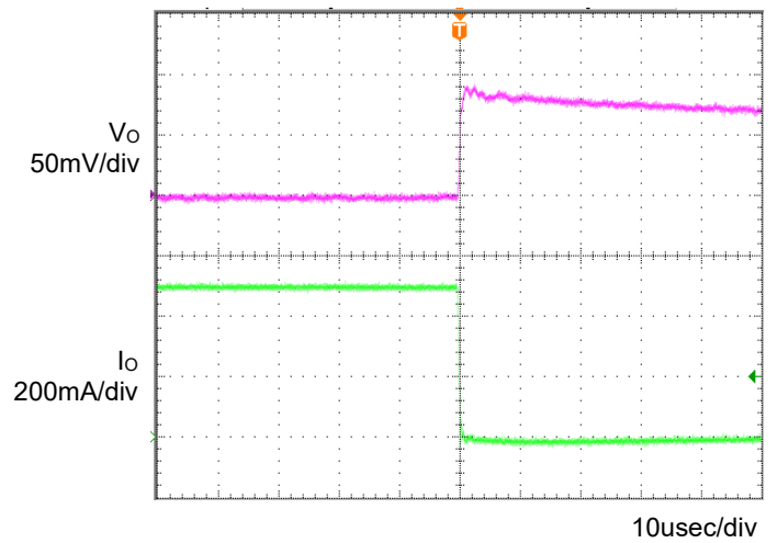
Fig.6 Transient Response (0.5→0A) Co=1µF, Ta=-40°C
