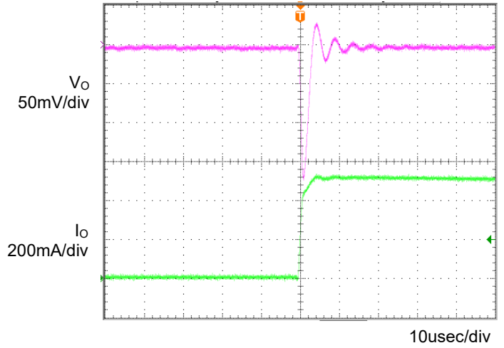
Fig.4 Transient Response (0→0.5A) Co=1µF, Ta=25°C
