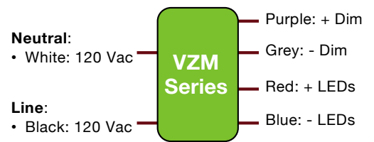
Wiring Diagram
