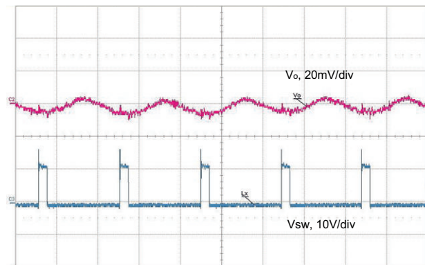
Fig. 55 - Output Ripple, 6 A, t = 1\text{ }\mu s/div Forced Continuous Conduction Mode
