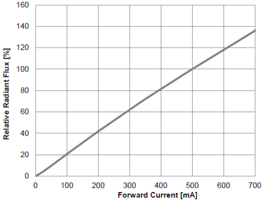
Fig 3. Relative Radiant Flux vs. Forward Current, T_a=25^\circ\text{C}
