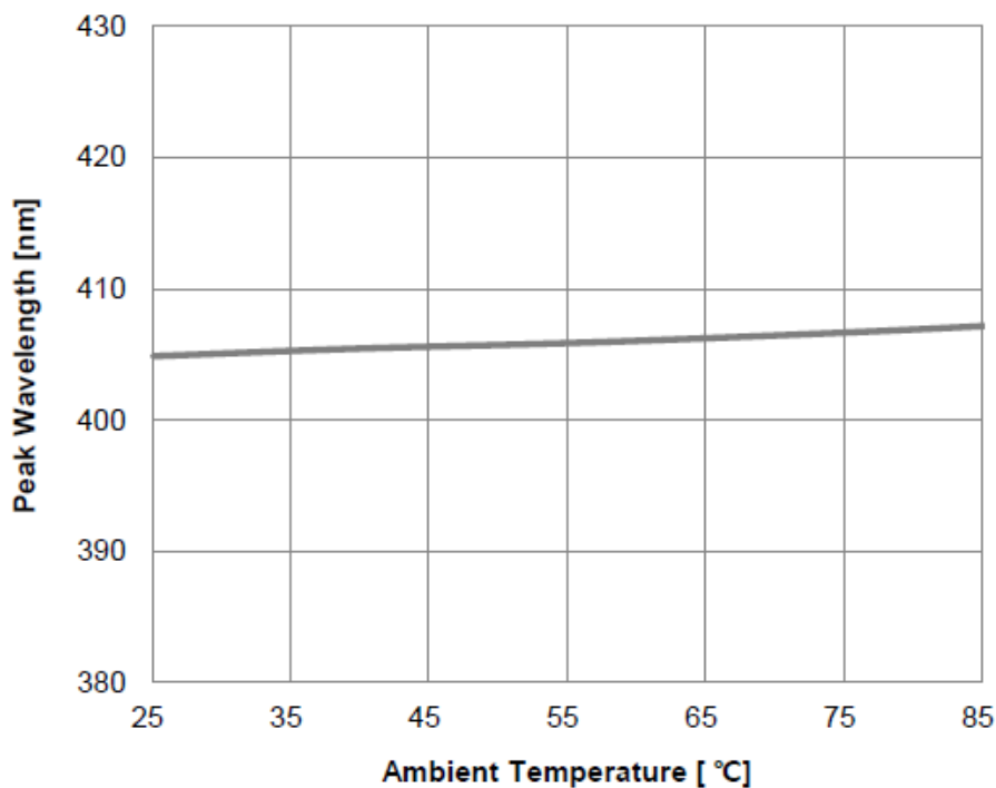
Fig 6. Peak Wavelength vs. Ambient Temperature, I_F=500mA
