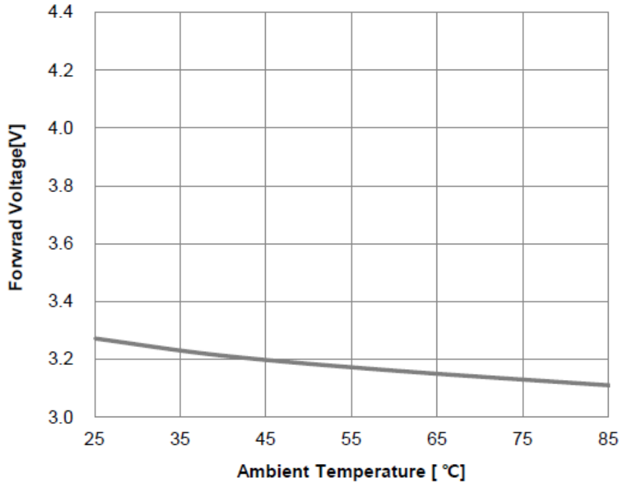
Fig 7. Forward Voltage vs Ambient Temperature, I_F=500mA
