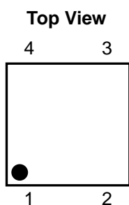
RP173K [DFN(PLP)1010-4] Pin Configuration
