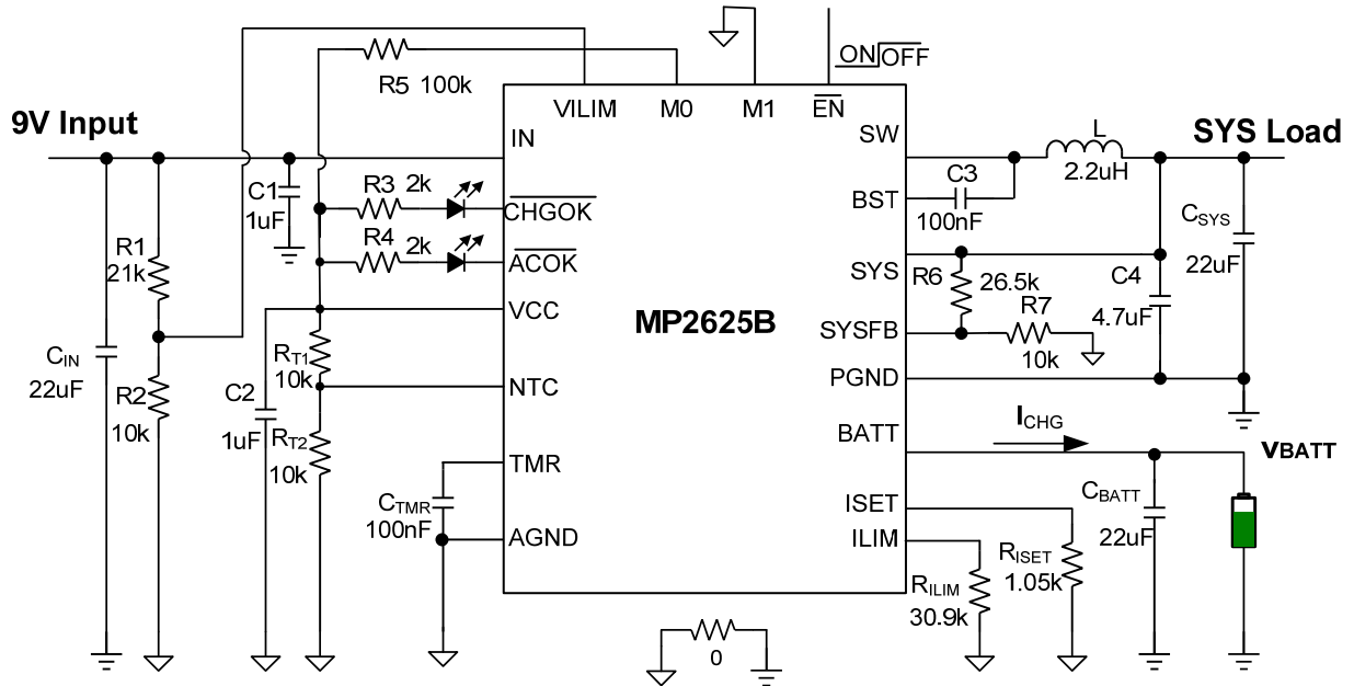
Figure 11: Typical Charge Application Circuit for 9V Input and 1.5A Input Current Limit
