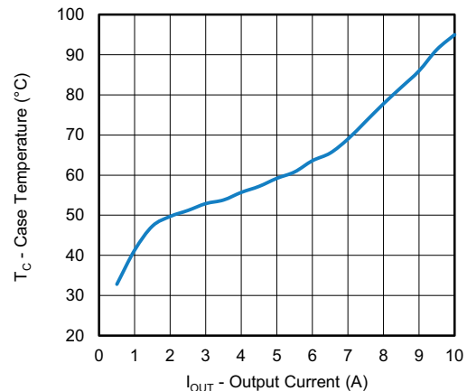
Fig. 15 - SiC466 Load Current vs. Case Temperature, V_{IN} = 48\text{ V} , V_{OUT} = 12\text{ V}
