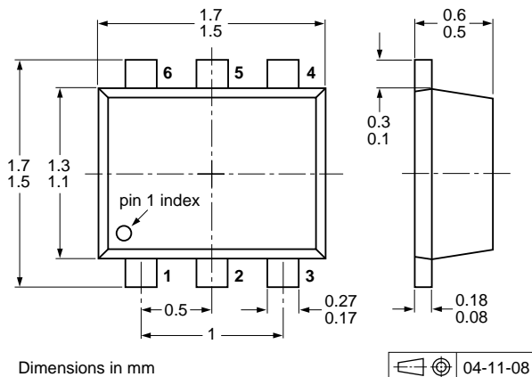
Fig 10. Package outline PEMH1 (SOT666)
