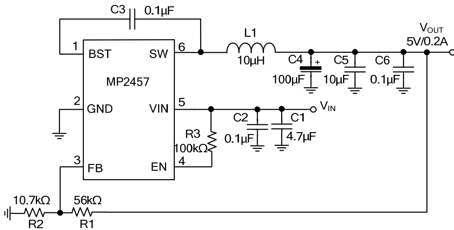
Figure 5: 5V Output
